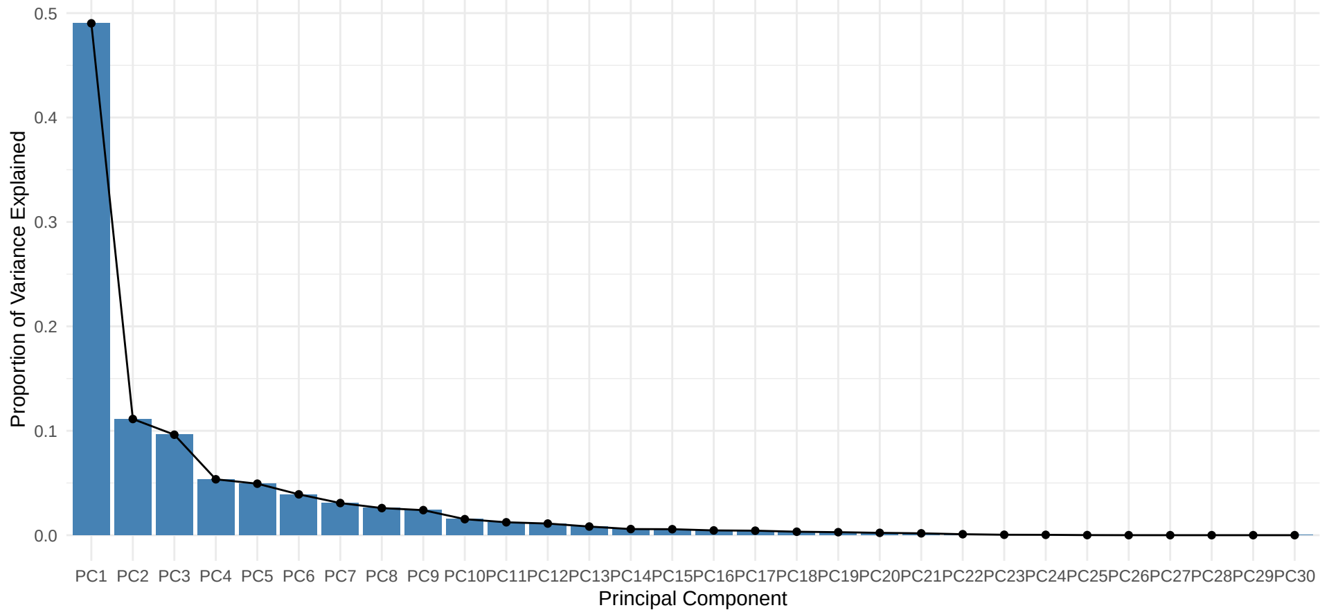
Scree Plot of PCA for FLARE003
